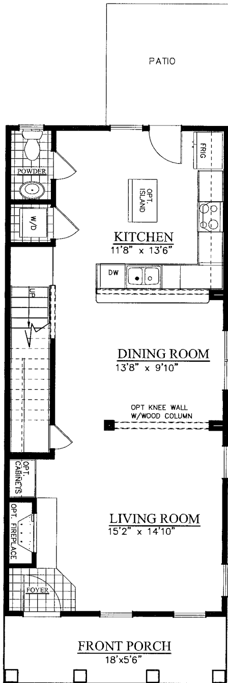
1ST FLOOR
