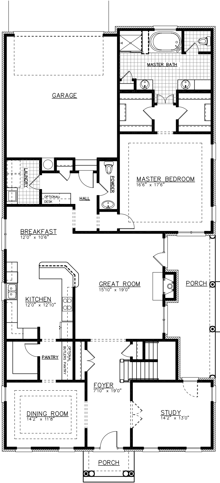
B1 STANDARD FIRST FLOOR
