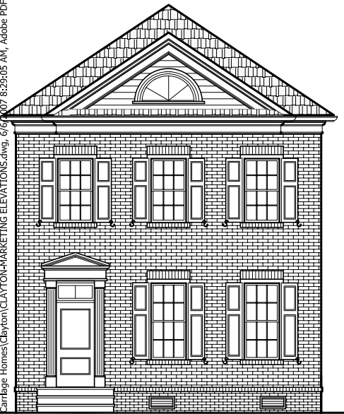
B1 STANDARD ELEVATION
