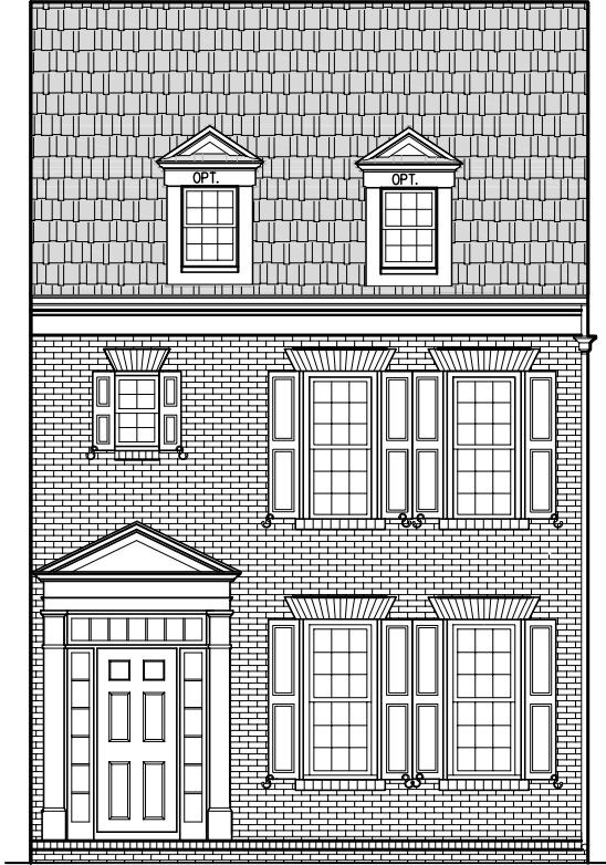
B4 ELEVATION
