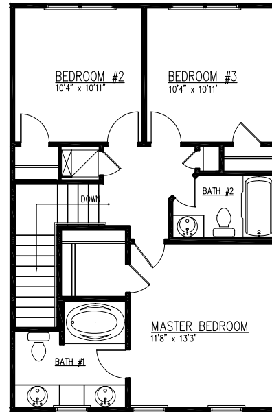
THIRD FLOOR
