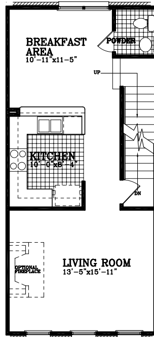
SECOND FLOOR
