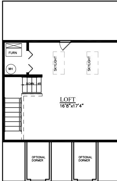
3RD FLOOR
