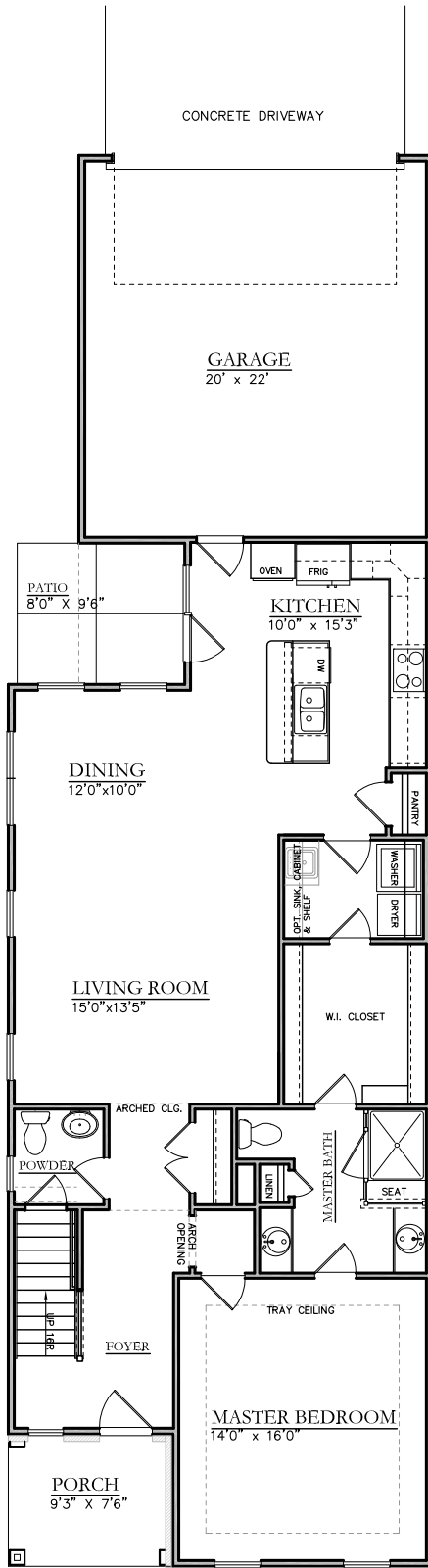
1ST FLOOR
