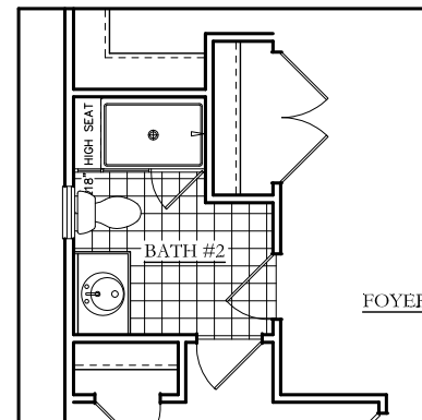
OPT. FIRST FLOOR SHOWER
