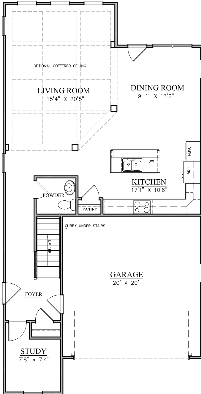
1ST FLOOR
