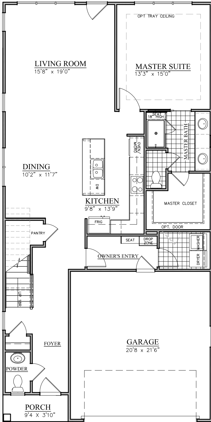
1ST FLOOR
