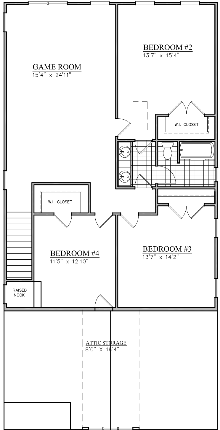
2ND FLOOR
